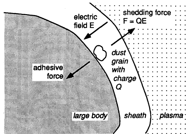
Fig. 1 Sketch of forces acting on a dust particulate attached to a large body (not to scale).
